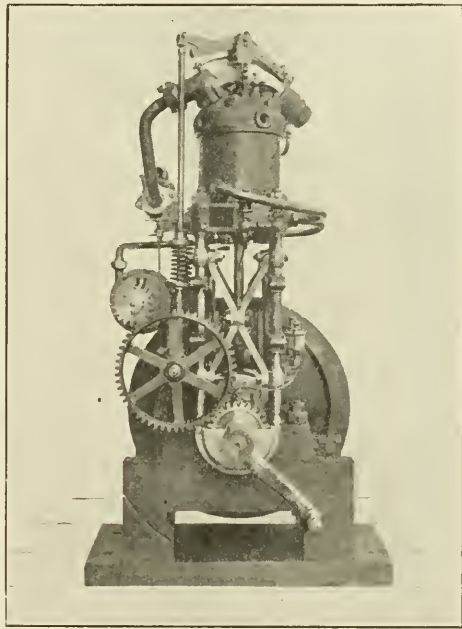
Fig. 12. Independent Auxiliary Gasoline-Driven Air Compressor.
